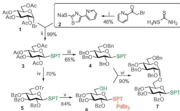
Scheme 2 Synthesis/evaluation of SPT donor 4 and acceptor 6 . Reagents and conditions: (i) Na/MeOH; (ii) MeCN; (iii) 1. MeONa/MeOH, 2. BnBr/NaH, DMF; (iv) 1. NaOMe/MeOH, 2. TrCl, C 3 H 5 N, 3. BzCl; (v) 1. PdBr 2 , 3 Å MS, 1,2-DCE, 2. 10% TFA/wet DCM, 0 °C; (vi) 1. AgOTf, 3 Å MS, DCM, 2. NaCN, acetone.
