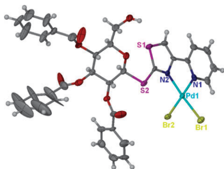
Fig. 2 X-Ray crystal structure of the acceptor complex 6 . Projection view of the molecule with 50% thermal ellipsoids—the disordered component and solvent have been omitted for clarity. Selected crystallographic parameters for 6 : Empirical formula C 38 H 36 Br 2 N 2 O 10 PdS 2 ; formula weight 1011.03; monoclinic; space group C2, Z = 4. Unit cell dimensions: a = 26.134(2), b = 6.6651(5), c = 26.550(3) Å, β = 118.580(4)°, volume 4061.1(7) Å 3 ; number of reflections collected 41 064; independent reflections 7012 [R(int) = 0.064]; final R indices: R1 [I > 2σ(I)] = 0.0431, wR2 (all data) = 0.0951. CCDC # 693543.
