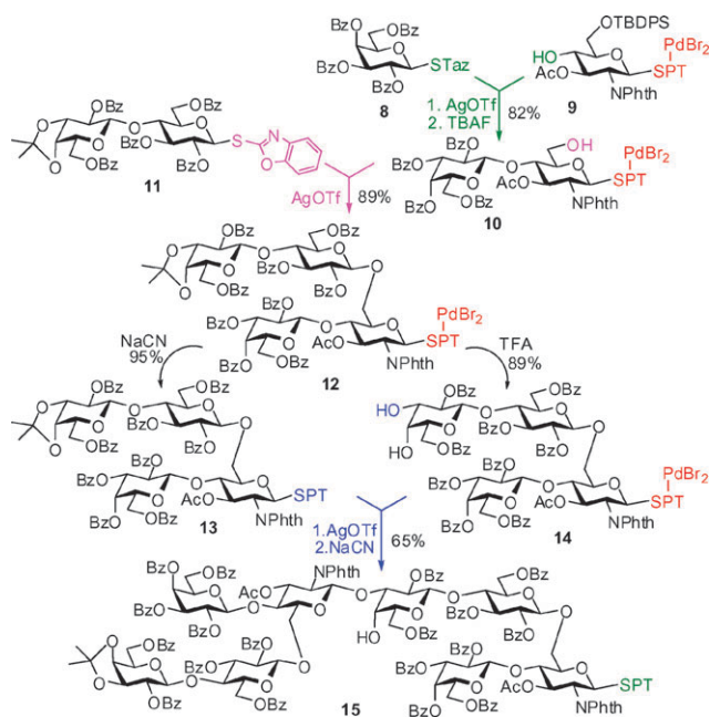
Scheme 3 Synthesis of pneumococcal oligosaccharides.
